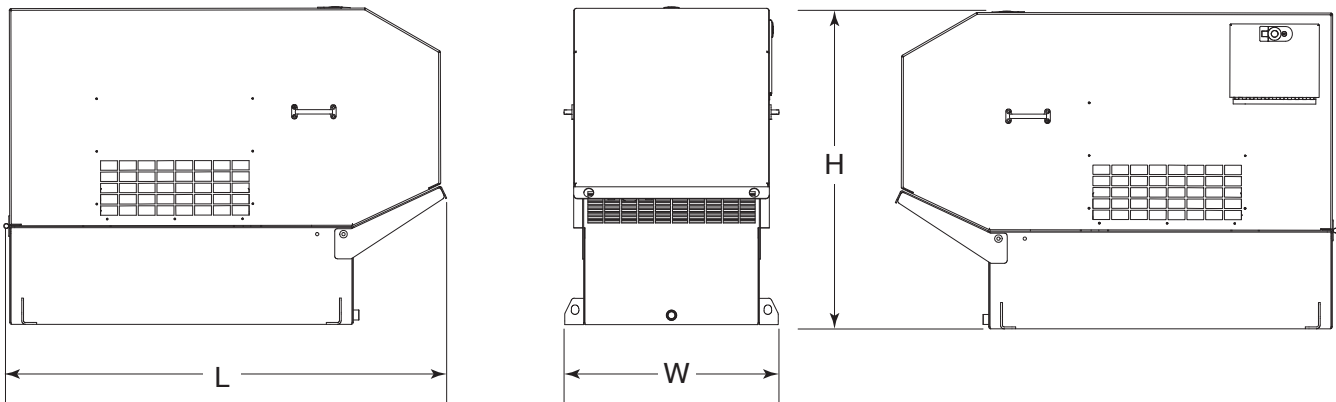
DIMENSIONS & ARRANGEMENT DRAWING MOBILE MODEL (WITH ENCLOSURE OPTION): TP9 T4i
