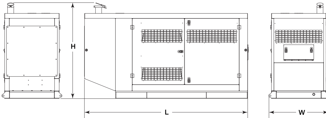
DIMENSIONS & ARRANGEMENT DRAWING MODEL: TG150
