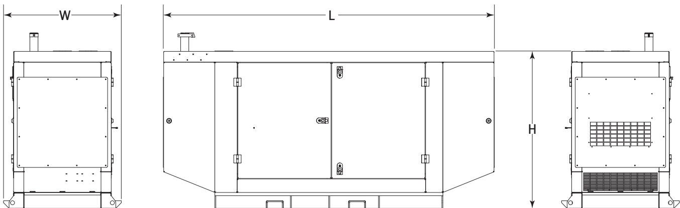
DIMENSIONS & ARRANGEMENT DRAWING MODEL: TG45
