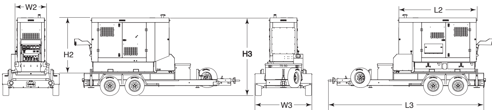
DIMENSIONS & ARRANGEMENT DRAWING MOBILE MODEL (WITH DOT TRAILER & ENCLOSURE OPTION): TDE80 T4
