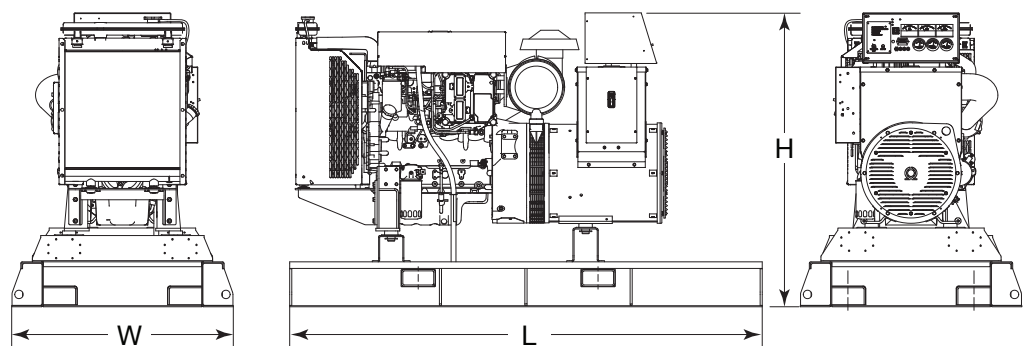
ARRANGEMENT DRAWING MODEL: TP56P
